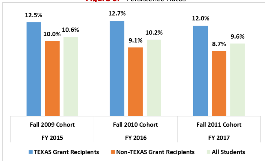
Figure 6. Persistence Rates
